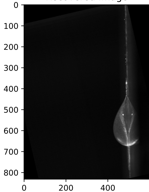
Recovered Image
