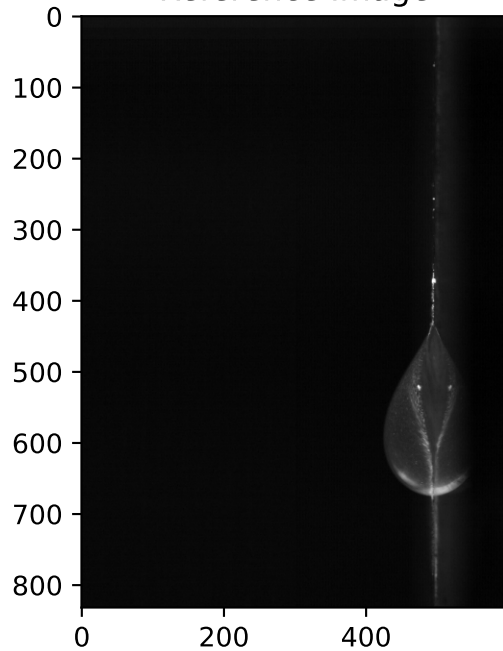
Reference Image
