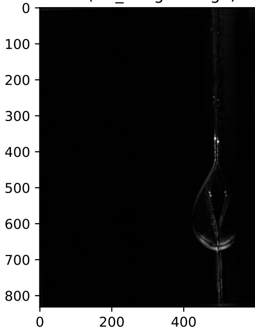
\text{abs}(\text{ref\_image}-\text{image})
