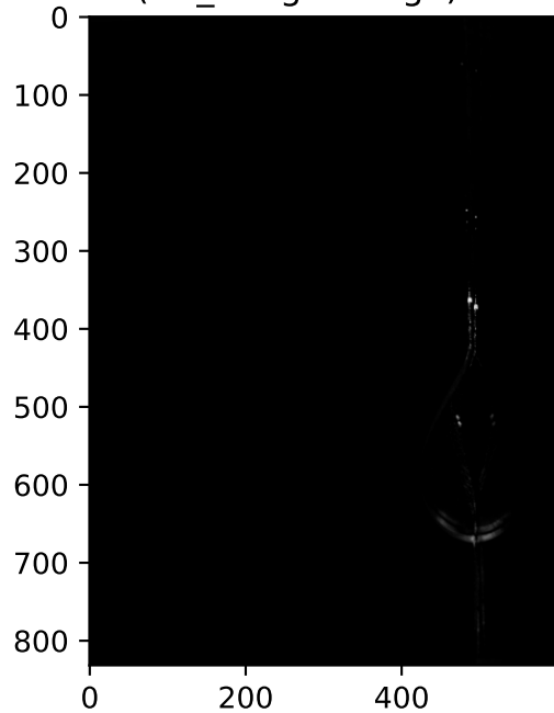
(\text{ref\_image}-\text{image})^2
